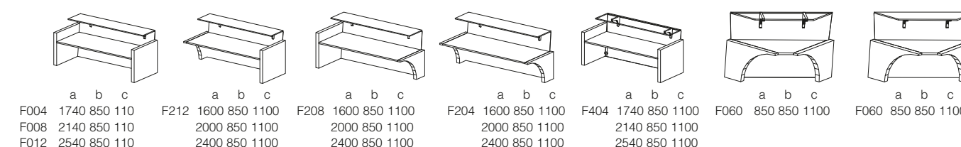
Recepciós pultok / Empfangstheken / Reception desks
